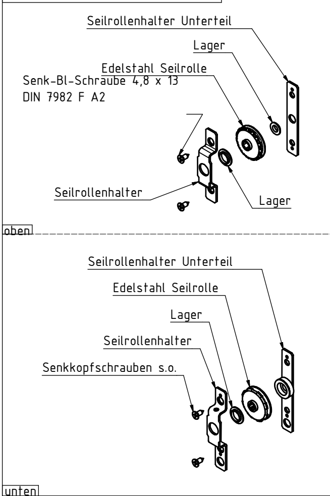
Rundmastkopf
